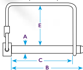
SHAFT LOCKING PIN Square Type-Mild Steel, Zinc Yellow Suitable for Square Shafts up to 2" Dia.
